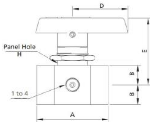
4-way Valve
