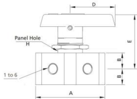
6-way Valve
