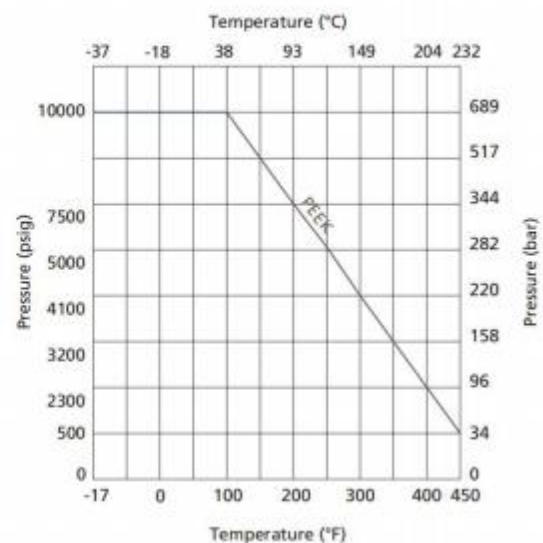
TBVH Series
